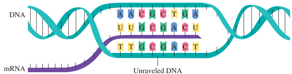
FIGURE 24.16 ▲ Formation of messenger RNA (transcription)
