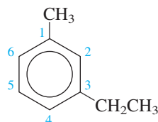
3-Ethyl-1-methylbenzene
