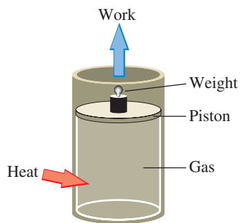
FIGURE 18.2 ▲ Exchanges of heat and work with the surroundings
