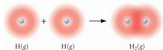
FIGURE 9.10 ▲ The electron probability distribution for the H 2 molecule
