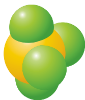
FIGURE 10.10 ▲ The sulfur tetrafluoride molecule Molecular model.
