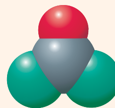
\text{COCl}_2
