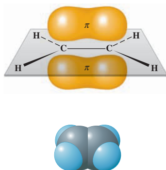
FIGURE 23.8 ▲ Representations of the ethylene molecule Top: Pi bonding forces the two CH_2 groups in ethylene to bond so as to give a planar structure. Bottom: A space-filling model shows the planar structure of the molecule.
