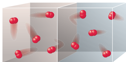
FIGURE 6.5 ▲ A kinetic-theory explanation of heat
