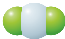
BeF 2
