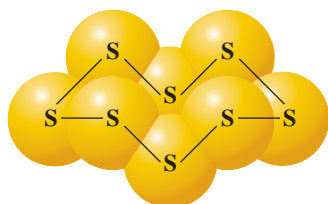
S 8
