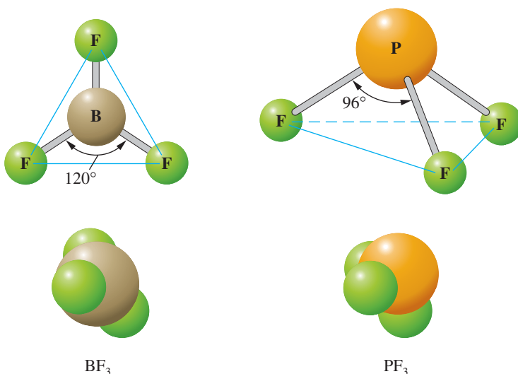
FIGURE 10.1 ▲ Molecular models of \text{BF}_3 and \text{PF}_3
