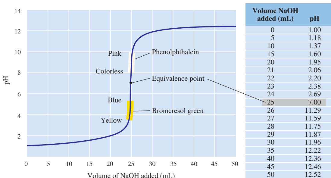
FIGURE 16.12 ▲ Curve for the titration of a strong acid by a strong base
