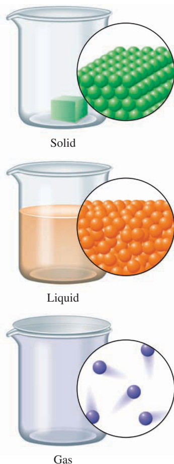
FIGURE 1.11 ▲ Molecular representations of solid, liquid, and gas
