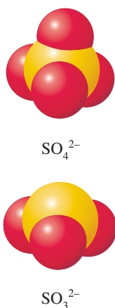
FIGURE 2.25 ▲ Sulfate and sulfite oxoanions
