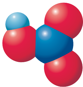
FIGURE 2.26 ▲ Molecular model of nitric acid
