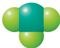
FIGURE 10.11 ▲ The chlorine trifluoride molecule Molecular model.
