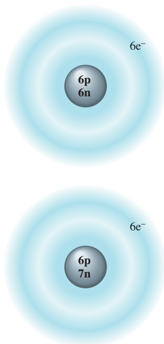
FIGURE 2.9 ▲ A representation of two isotopes of carbon
