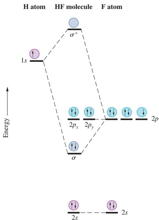
FIGURE 10.35 ▲ Relative energies of molecular orbitals in the valence shell of HF
