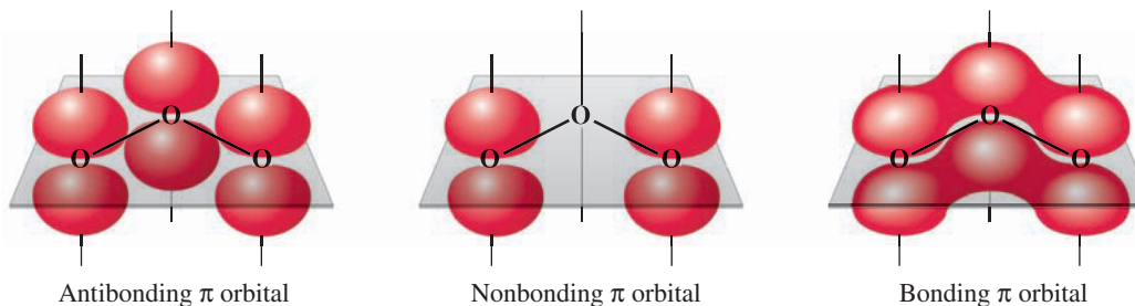
FIGURE 10.37 ▲ The electron distributions of the \pi molecular orbitals of O_3
