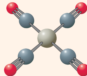
\text{Ni}(\text{CO})_4
