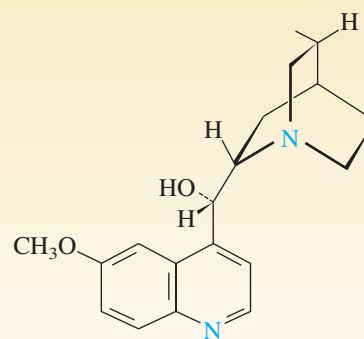
Quinine (antimalarial)
