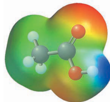
FIGURE 3.1 ▲ Electrostatic potential map of acetic acid molecule (CH 3 COOH)
