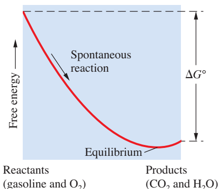
FIGURE 18.11 ▲ Free-energy change during a spontaneous reaction (combustion of gasoline)
