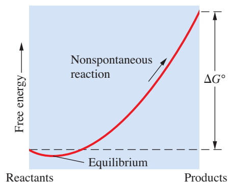
FIGURE 18.12 ▲ Free-energy change during a nonspontaneous reaction
