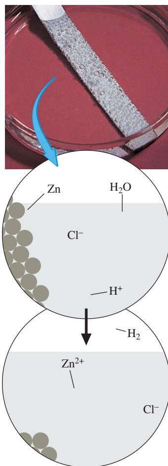
FIGURE 4.16 ▲ Displacement reaction
