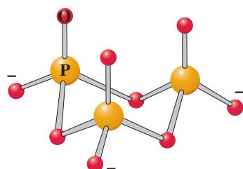
FIGURE 21.50 ▲ The structure of trimetaphosphate ion, \text{P}_3\text{O}_9^{3-}
