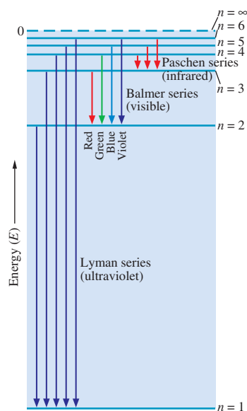
FIGURE 7.11 ▲ Transitions of the electron in the hydrogen atom
