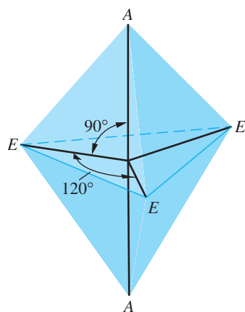
FIGURE 10.9 ▲ Trigonal bipyramidal arrangement of electron pairs
