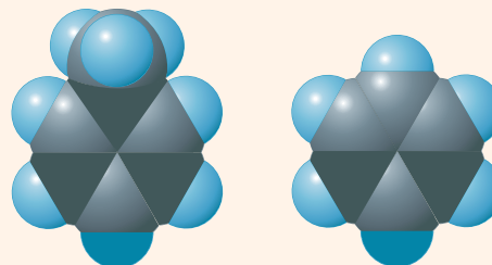
Toluene
