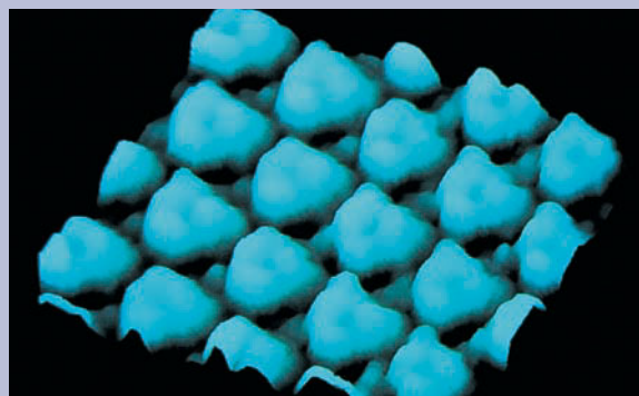
FIGURE 7.19 ▲ Scanning tunneling microscope image of benzene molecules on a metal surface
