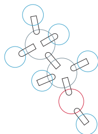
Ethanol C_2H_5OH
