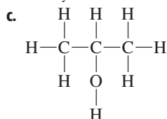
isopropyl alcohol
