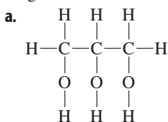
glycerol
