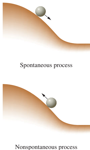
FIGURE 18.4 ▲ Examples of a spontaneous and a nonspontaneous process
