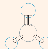
Formaldehyde \text{CH}_2\text{O}
