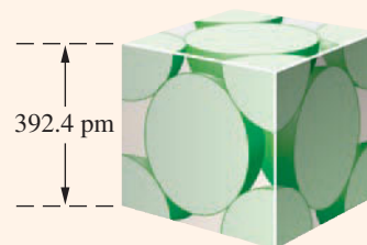
Platinum d = 21.45 g/cm 3 atomic mass = 195.08 amu
