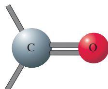
Carbonyl group
