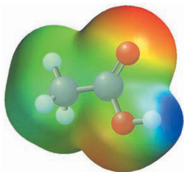
Acetic acid
