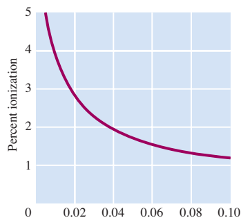
FIGURE 16.3 ▲ Variation of percent ionization of a weak acid with concentration
