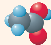
FIGURE 3.10 ▲ Molecular model of acetic acid
