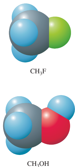
FIGURE 11.23 ▲ Fluoromethane and methanol Space-filling molecular models. (Top) fluoromethane, CH 3 F; (bottom) methanol, CH 3 OH.
