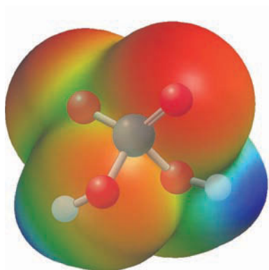
Sulfuric acid
