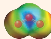
Ozone \text{O}_3
