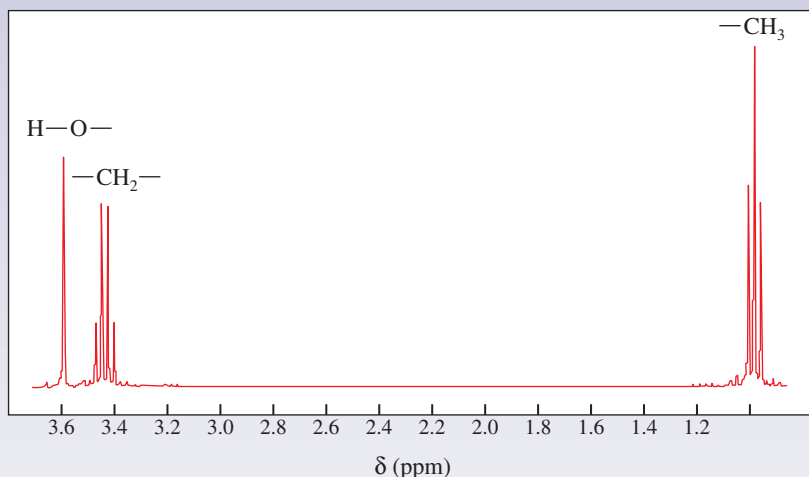
FIGURE 8.6 ▲ High-resolution NMR spectrum of ethanol, CH 3 CH 2 OH
