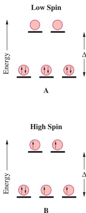
FIGURE 22.25 ▲ Occupation of the 3d orbitals in complexes of \text{Fe}^{2+} (A) Low spin. (B) High spin.
