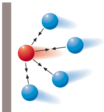
FIGURE 5.32 ▲ Effect of intermolecular attractions on gas pressure
