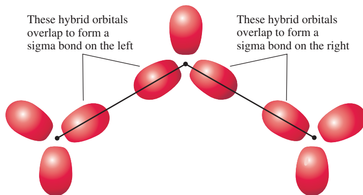
FIGURE 10.36 ▲ Hybrid orbitals on oxygen atoms of ozone, O_3
