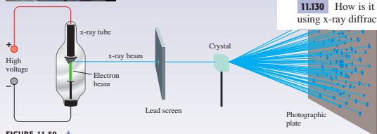
FIGURE 11.50 ▲ Automated x-ray diffractometer
