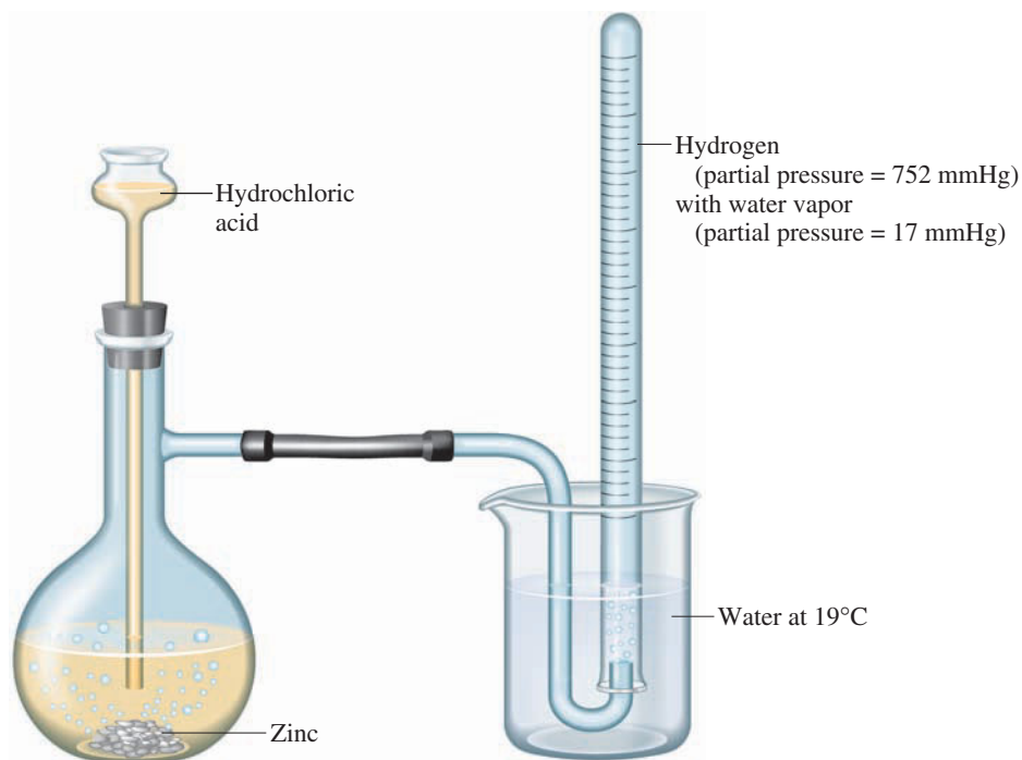
FIGURE 5.20 ▲ Collection of gas over water
