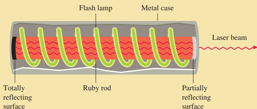
FIGURE 7.13 ▲ A ruby laser
