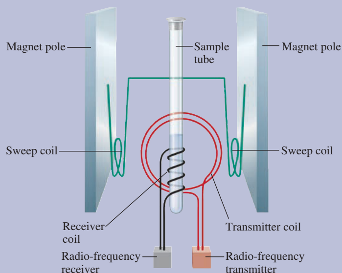
FIGURE 8.5 ▲ Nuclear magnetic resonance spectrometer
