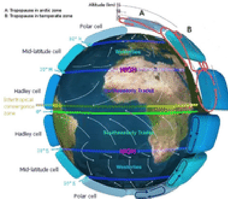
The direction of major wind belts
