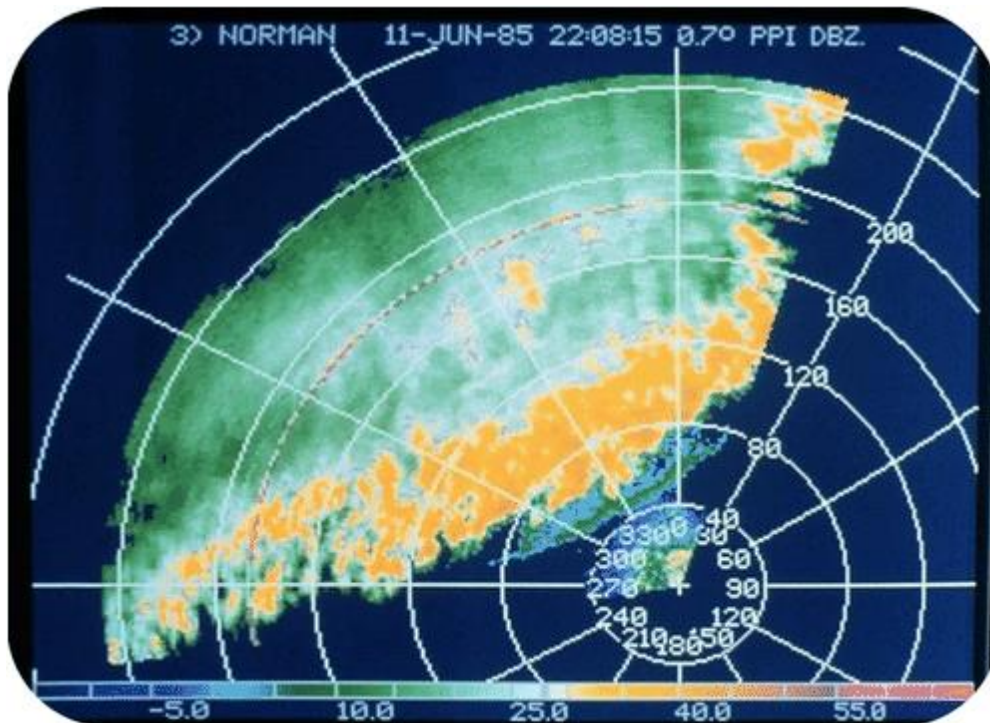
Radar image of a line of thunderstorms
