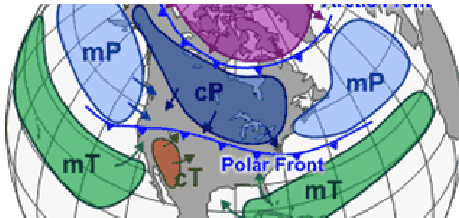
North American air masses
