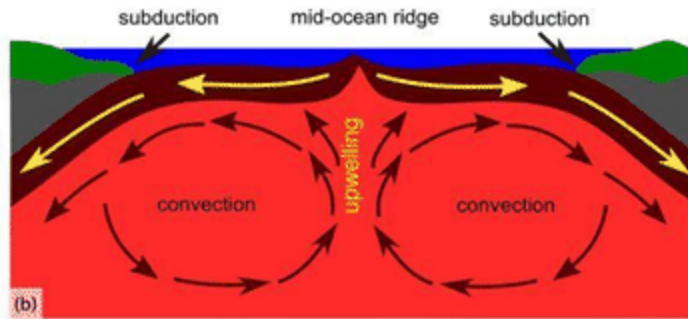
Diagram of convection within Earth's mantle.
