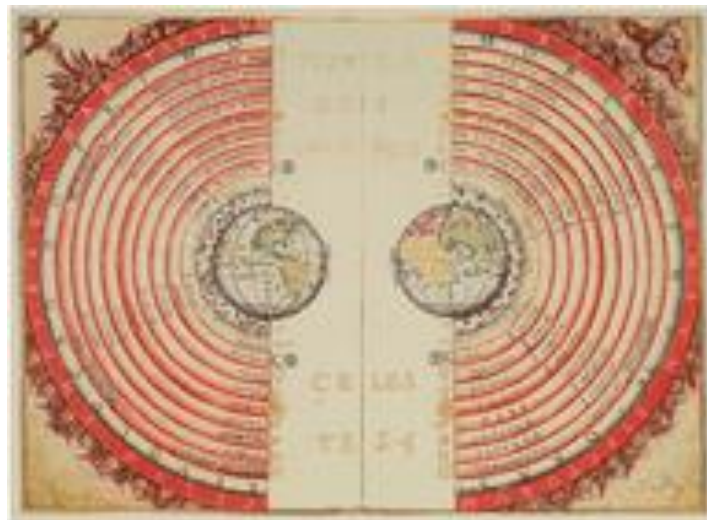
Timeline of cosmological theories
